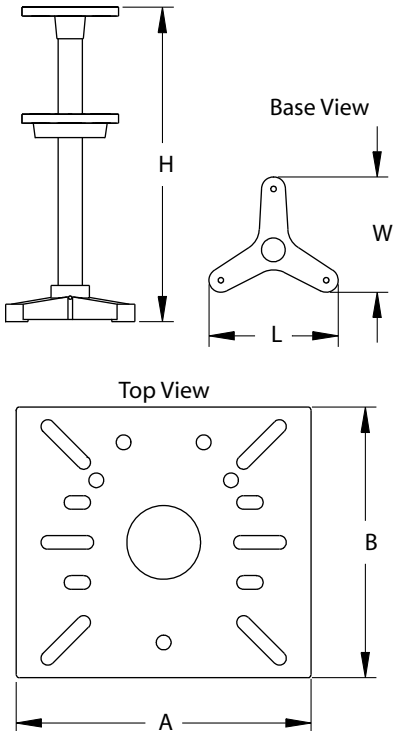
Figure 1 - Dimensions
